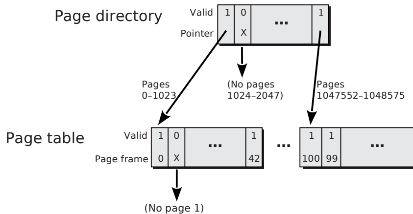
Figure 6.13: The IA-32 two-level page table has a page directory that can point to 1024 chunks of the page table, each of which can point to 1024 page frames. As in Fig. 6.11, entries (of page directory and page table) record valid bits and address information. For example, the leftmost entry of the leftmost chunk of the page table points to the page frame holding page 0, which is page frame 0; besides, page frame 42 holds page 1023, while page frames 100 and 99 hold pages 1047552 and 1047553, respectively. Each entry can also be marked invalid, indicated by a valid bit of 0 and an X in this diagram. For example, the second entry in the first chunk of the page table is invalid, showing that no page frame holds page 1. The same principle applies at the page directory level; in this example, no page frames hold pages 1024–2047, so the second page directory entry is marked invalid.
