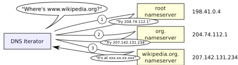
Figure 3: “Example of an iterative DNS resolver” by Lion Kimbro under Public domain; from Wikimedia
