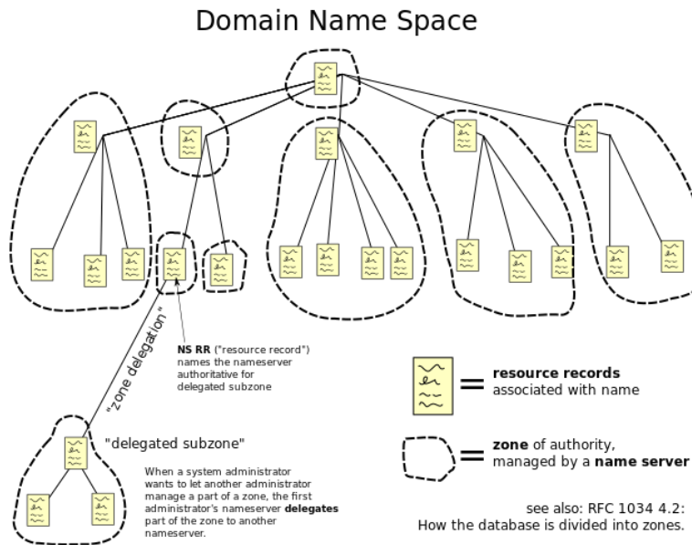
Figure 1: "Domain name space" by LionKimbrow under Public domain; from Wikimedia
