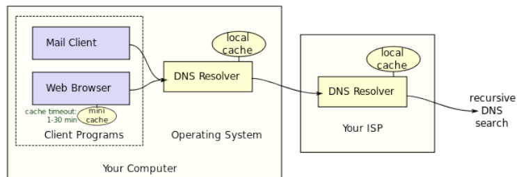
Figure 2: “DNS in the real world” by Lion Kimbro under Public domain ; from Wikimedia
